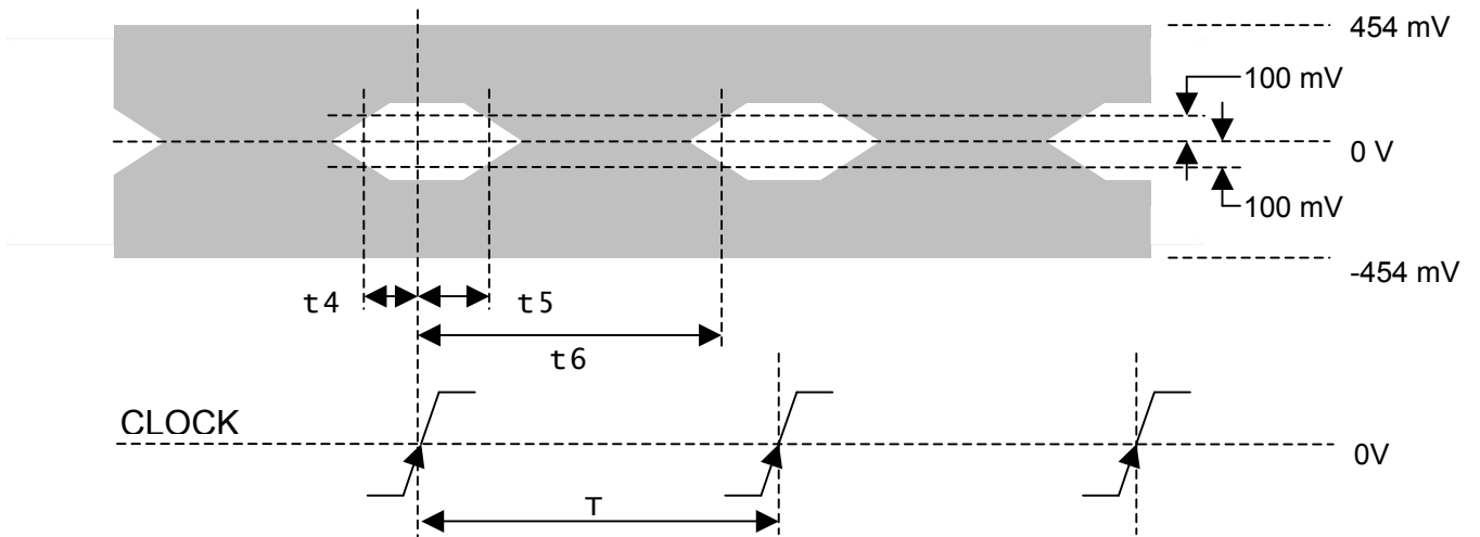
Figure 4: LVDS Receiver Input Eye Pattern
