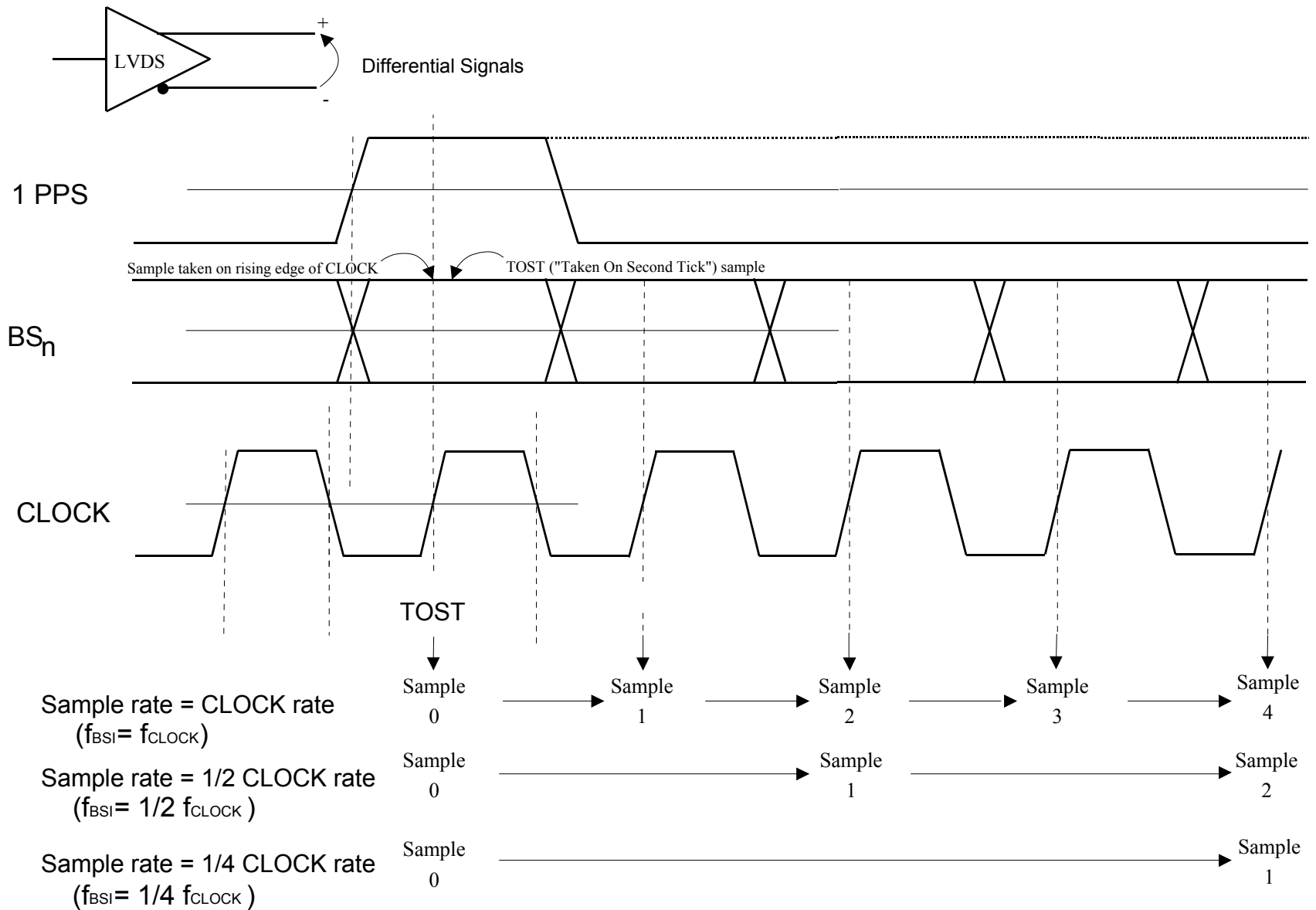
Figure 2: LVDS Timing Relationships
